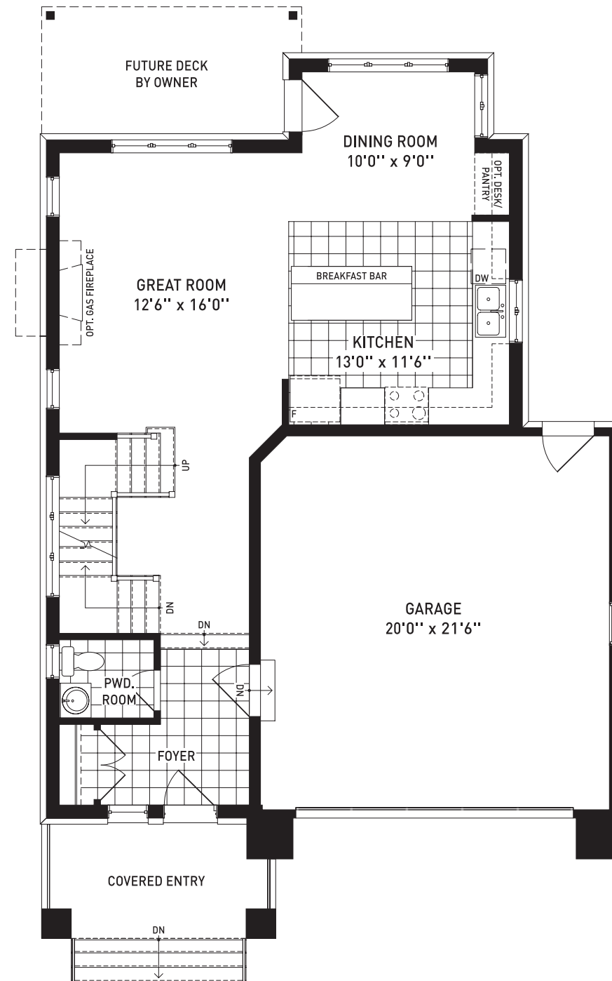
Ground Floor
