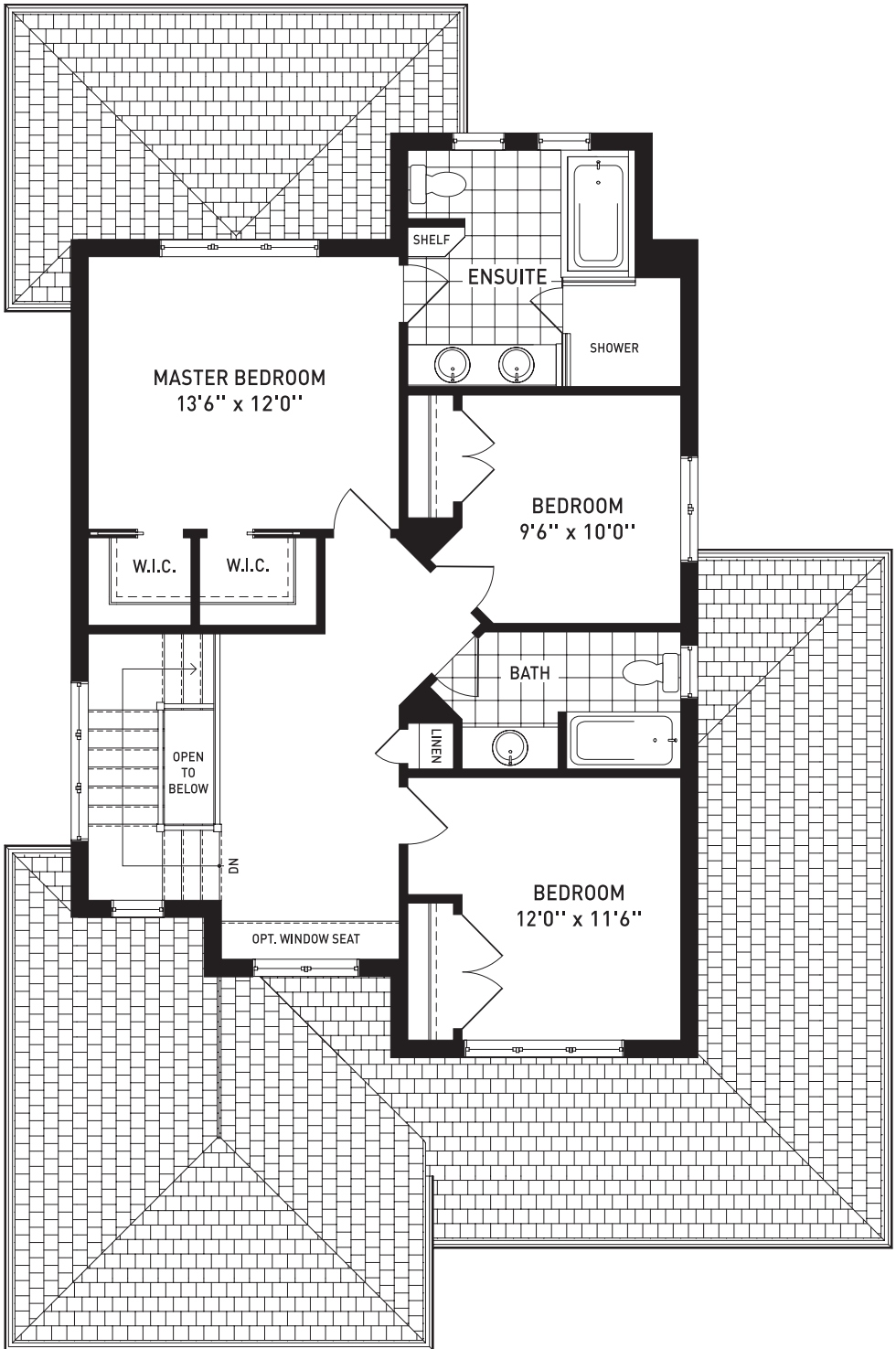
Second Floor
